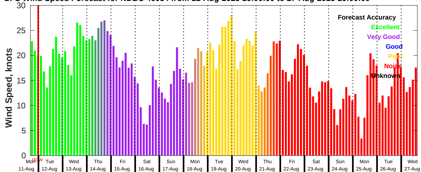
GFS Wind Speed Forecast for NDBC 46054 from 11-Aug-2025 16:00:00 to 27-Aug-2025 16:00:00
