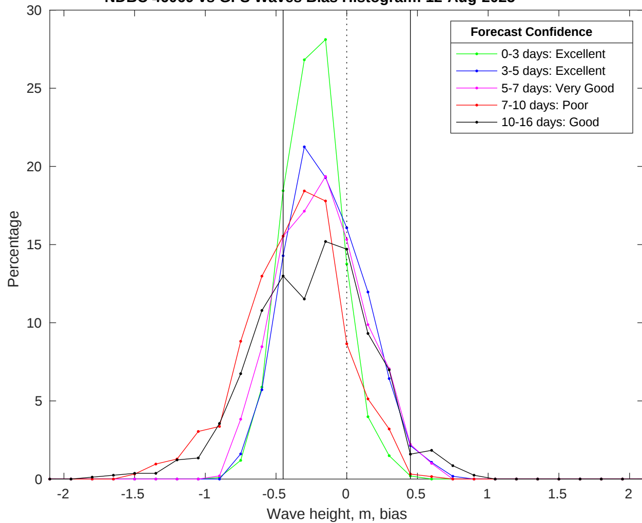
NDBC 46069 vs GFS Waves Bias Histogram: 12-Aug-2025
