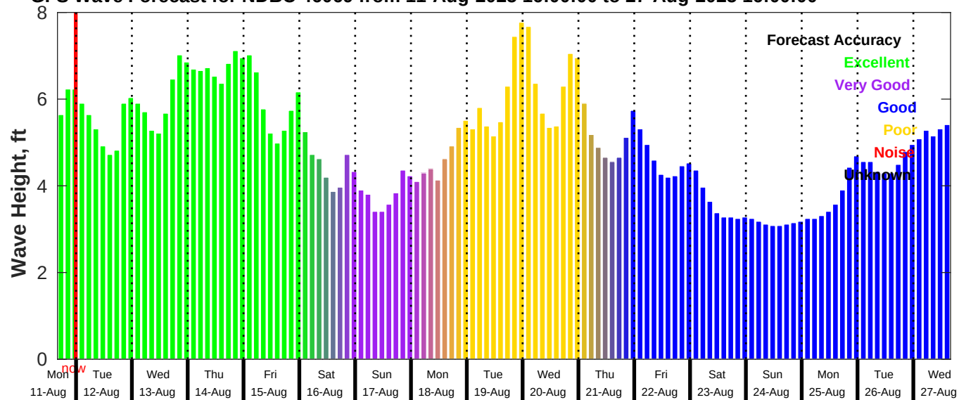
GFS Wave Forecast for NDBC 46069 from 11-Aug-2025 16:00:00 to 27-Aug-2025 16:00:00
