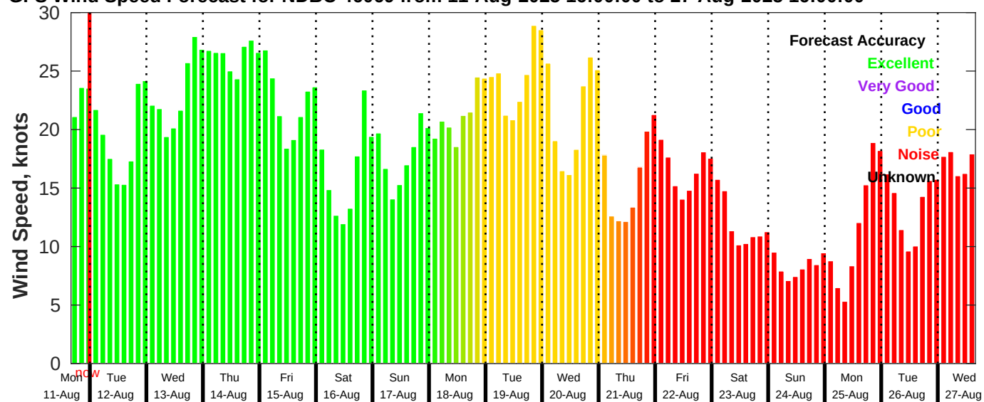
GFS Wind Speed Forecast for NDBC 46069 from 11-Aug-2025 16:00:00 to 27-Aug-2025 16:00:00
