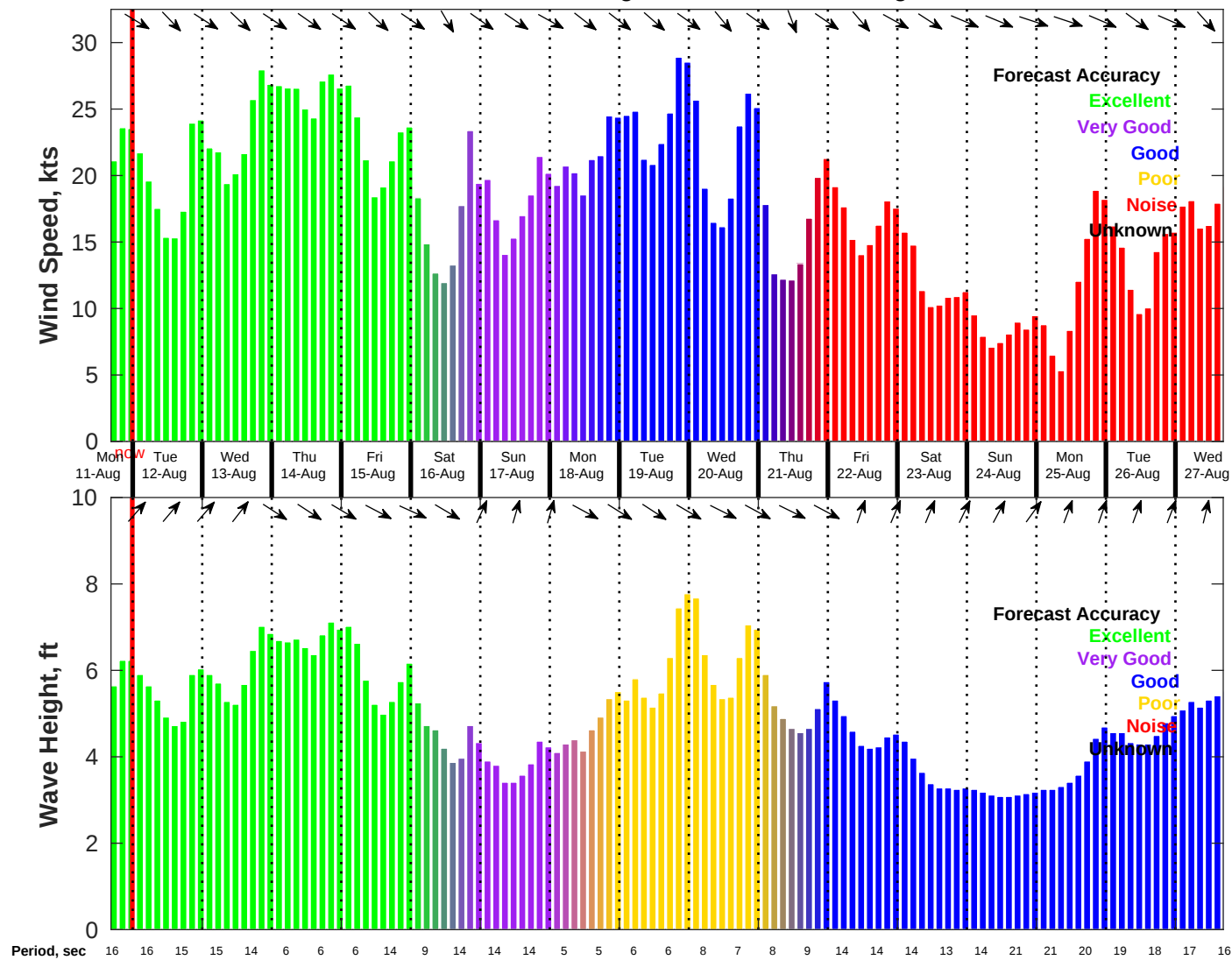
Wind & Wave Forecast for NDBC 46069 from 11-Aug-2025 16:00:00 to 27-Aug-2025 16:00:00
