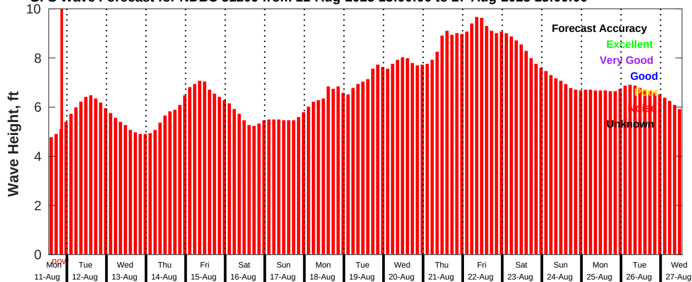
GFS Wave Forecast for NDBC 51209 from 11-Aug-2025 13:00:00 to 27-Aug-2025 13:00:00
