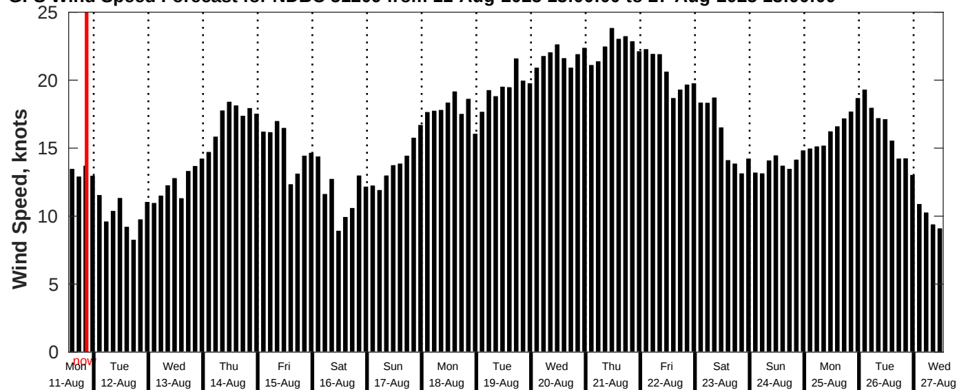
GFS Wind Speed Forecast for NDBC 51209 from 11-Aug-2025 13:00:00 to 27-Aug-2025 13:00:00
