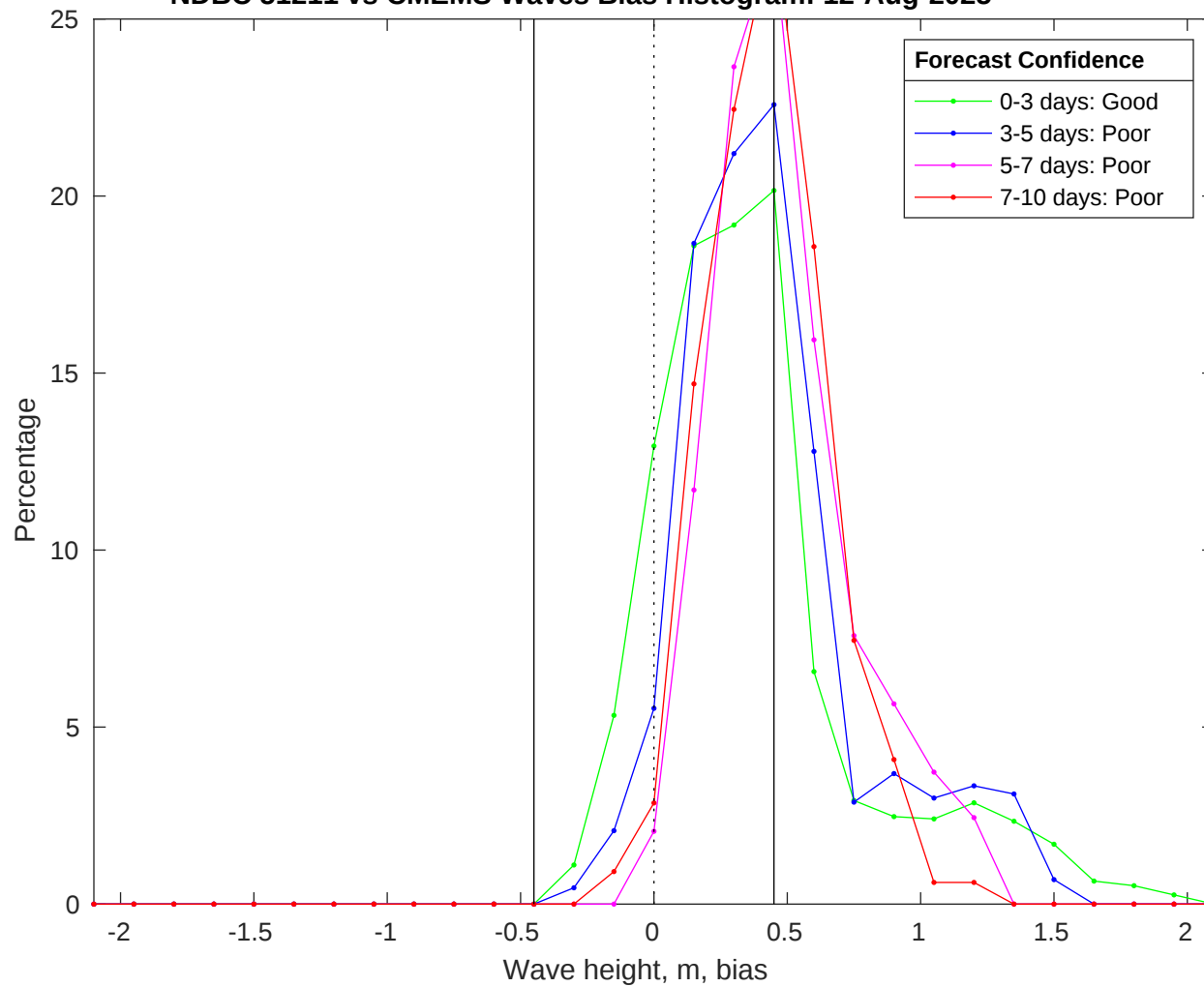
NDBC 51211 vs CMEMS Waves Bias Histogram: 12-Aug-2025
