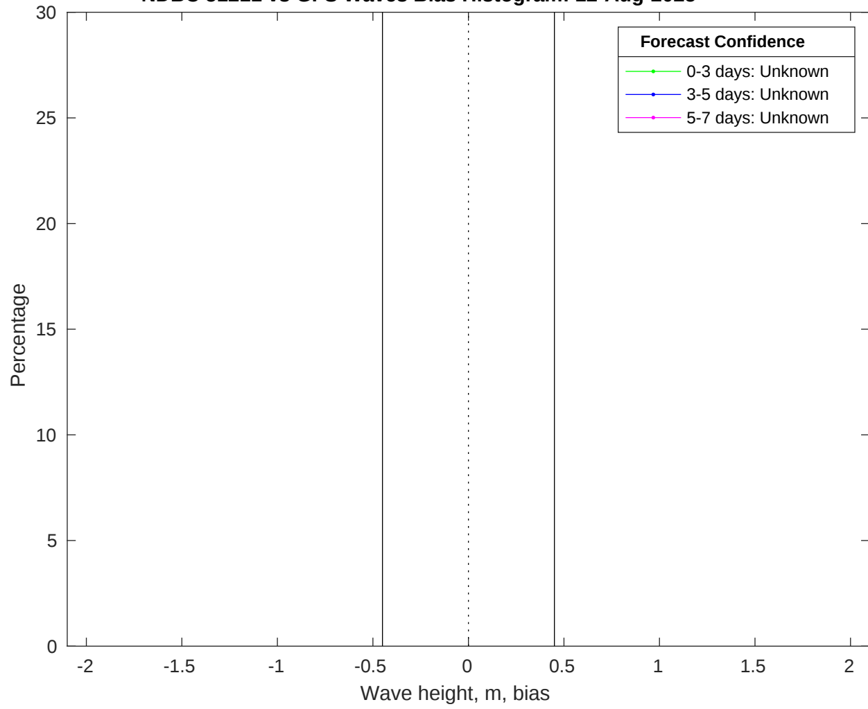
NDBC 51211 vs GFS Waves Bias Histogram: 12-Aug-2025
