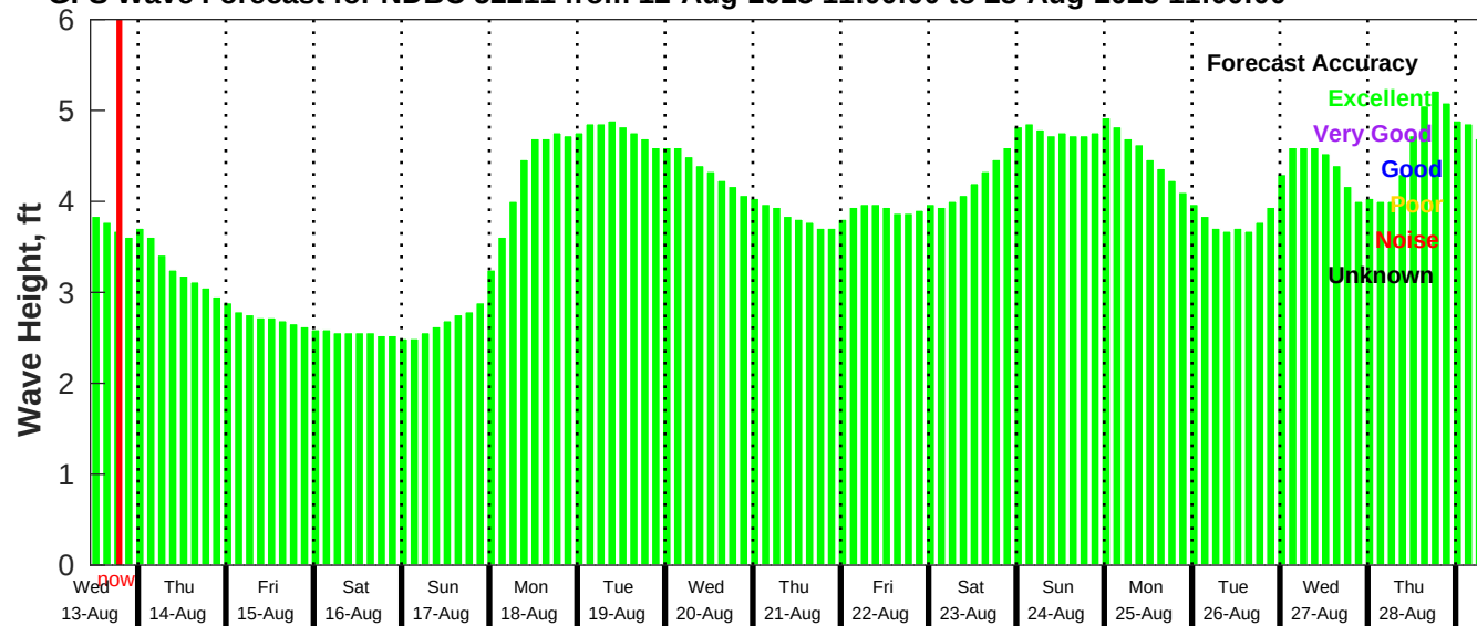
GFS Wave Forecast for NDBC 52211 from 12-Aug-2025 11:00:00 to 28-Aug-2025 11:00:00
