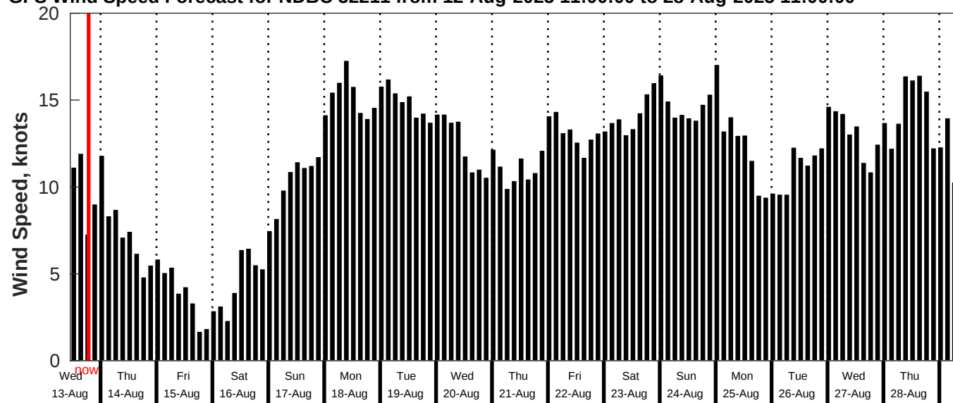
GFS Wind Speed Forecast for NDBC 52211 from 12-Aug-2025 11:00:00 to 28-Aug-2025 11:00:00
