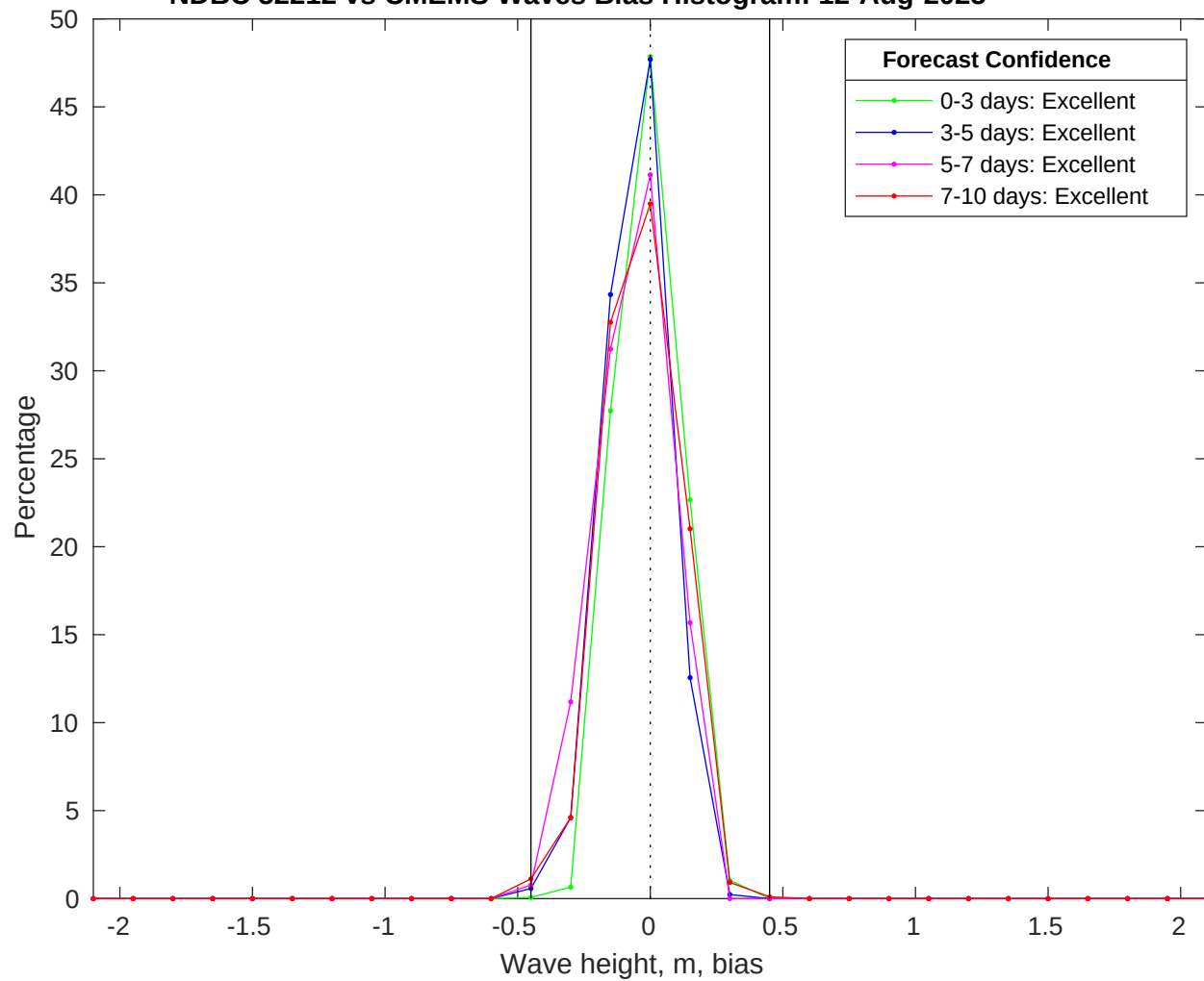
NDBC 52212 vs CMEMS Waves Bias Histogram: 12-Aug-2025
