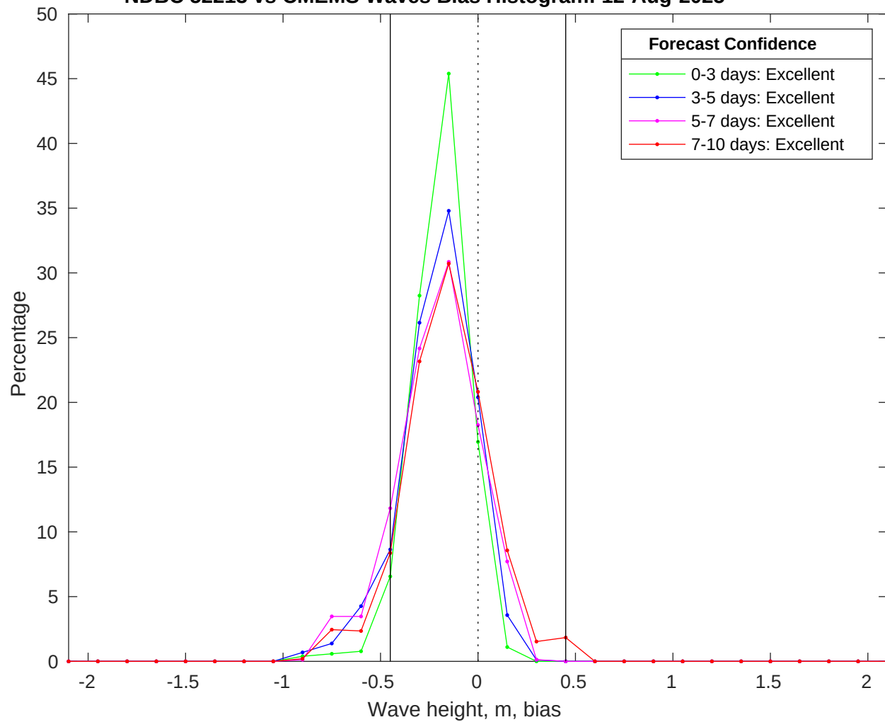
NDBC 52213 vs CMEMS Waves Bias Histogram: 12-Aug-2025
