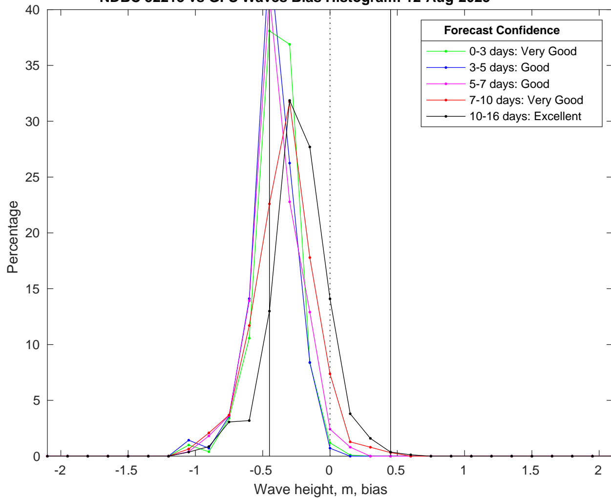
NDBC 52213 vs GFS Waves Bias Histogram: 12-Aug-2025
