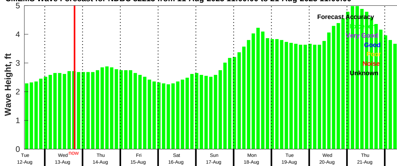
CMEMS Wave Forecast for NDBC 52213 from 11-Aug-2025 11:00:00 to 21-Aug-2025 11:00:00
