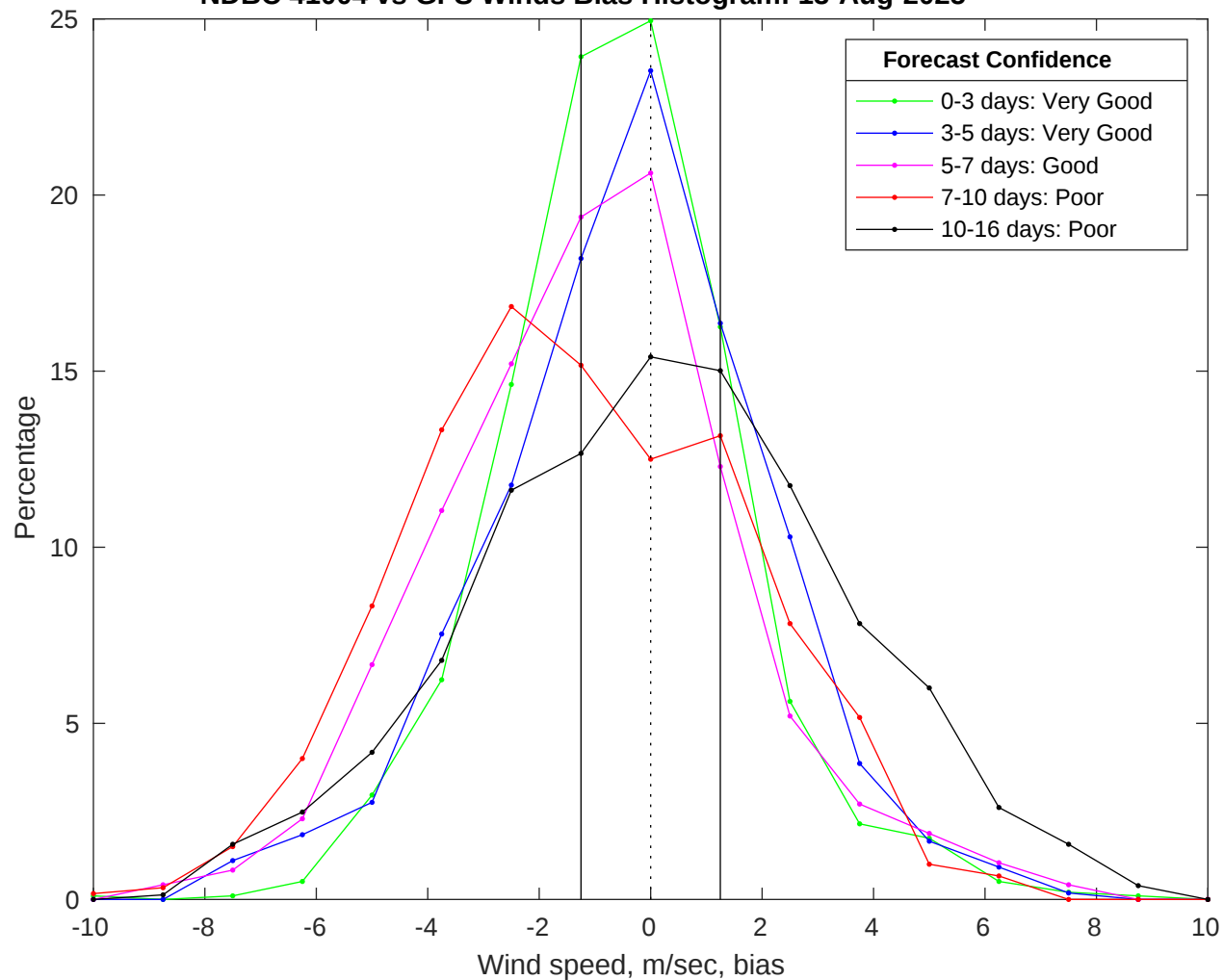
NDBC 41004 vs GFS Winds Bias Histogram: 13-Aug-2025
