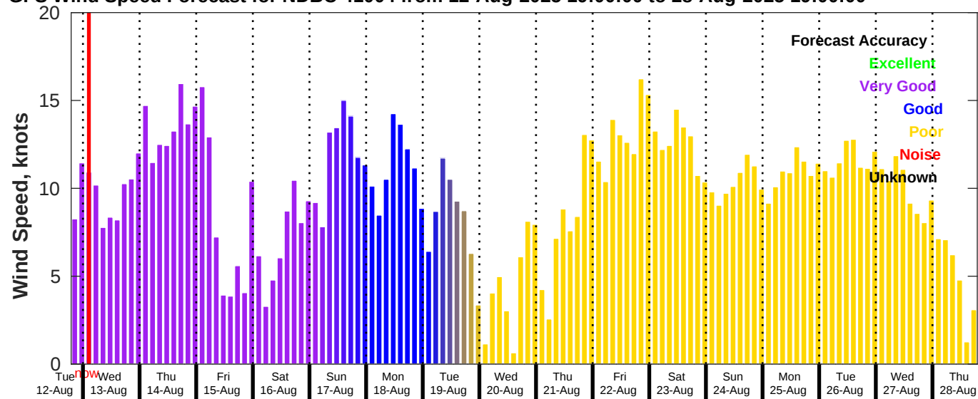
GFS Wind Speed Forecast for NDBC 41004 from 12-Aug-2025 19:00:00 to 28-Aug-2025 19:00:00
