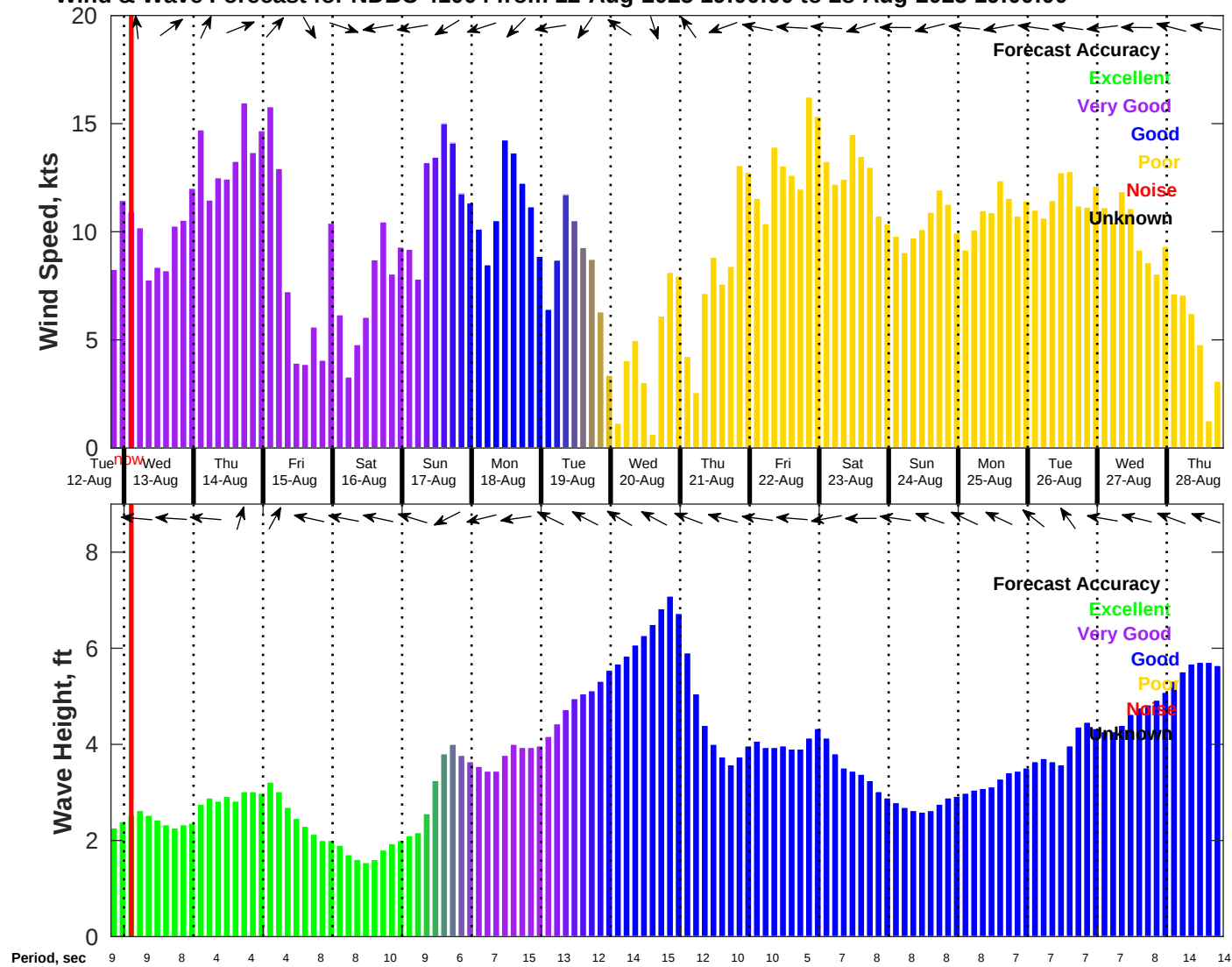
Wind & Wave Forecast for NDBC 41004 from 12-Aug-2025 19:00:00 to 28-Aug-2025 19:00:00
