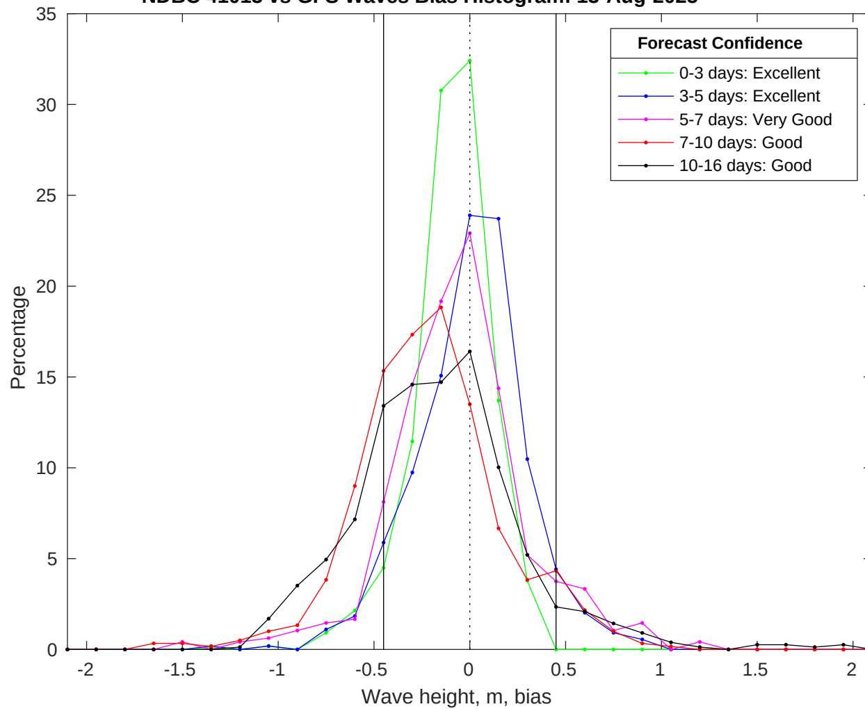
NDBC 41013 vs GFS Waves Bias Histogram: 13-Aug-2025
