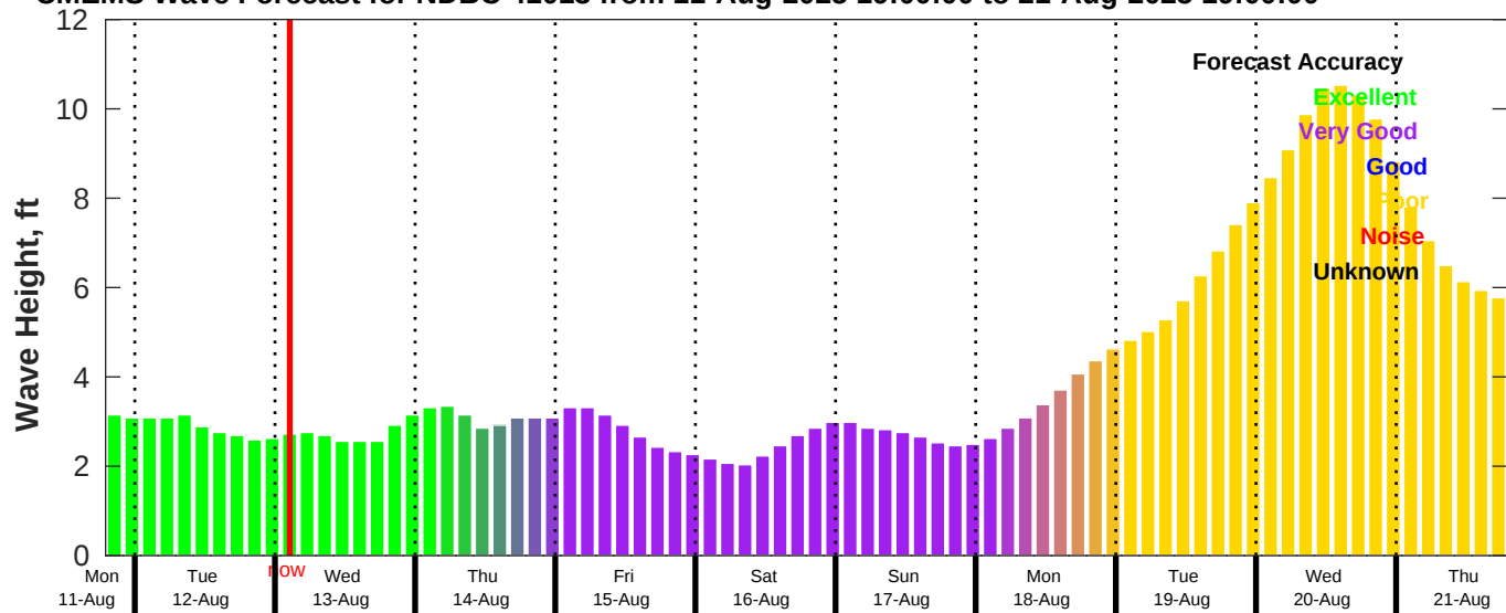
CMEMS Wave Forecast for NDBC 41013 from 11-Aug-2025 19:00:00 to 21-Aug-2025 19:00:00
