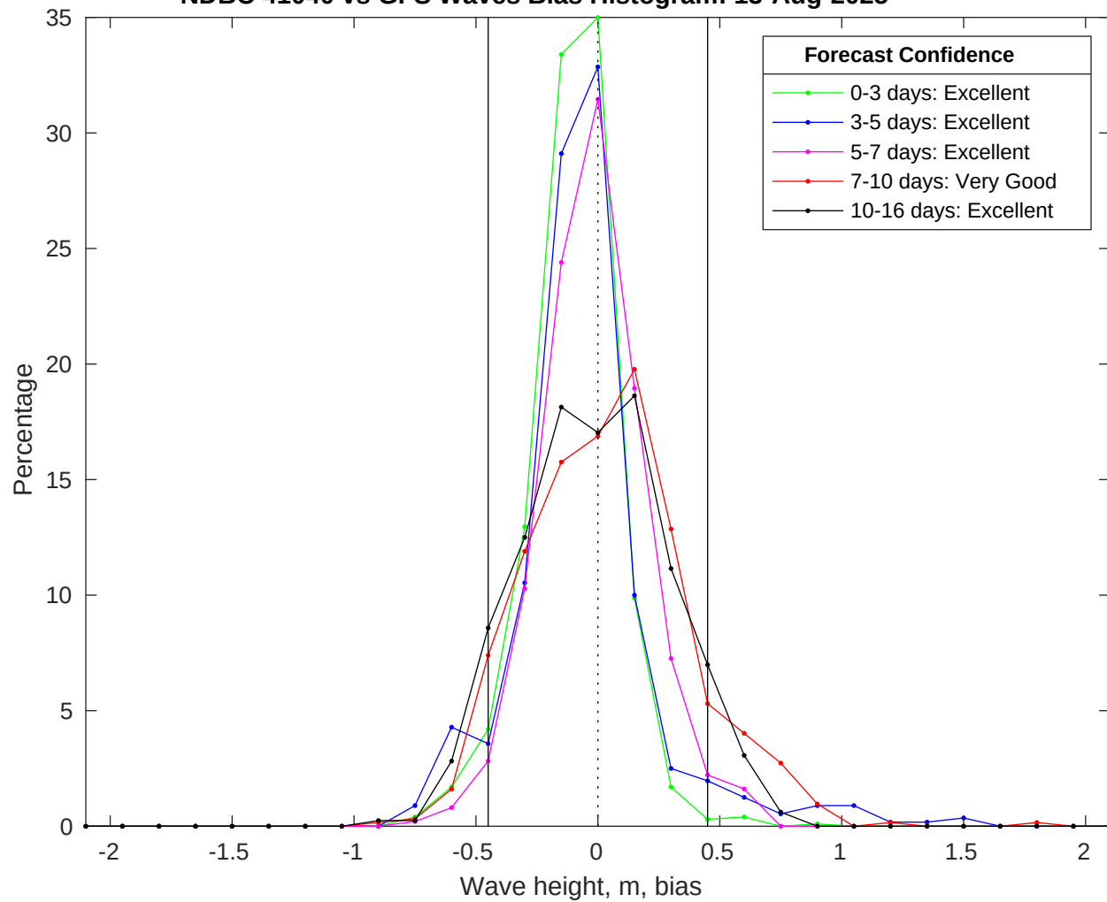
NDBC 41040 vs GFS Waves Bias Histogram: 13-Aug-2025
