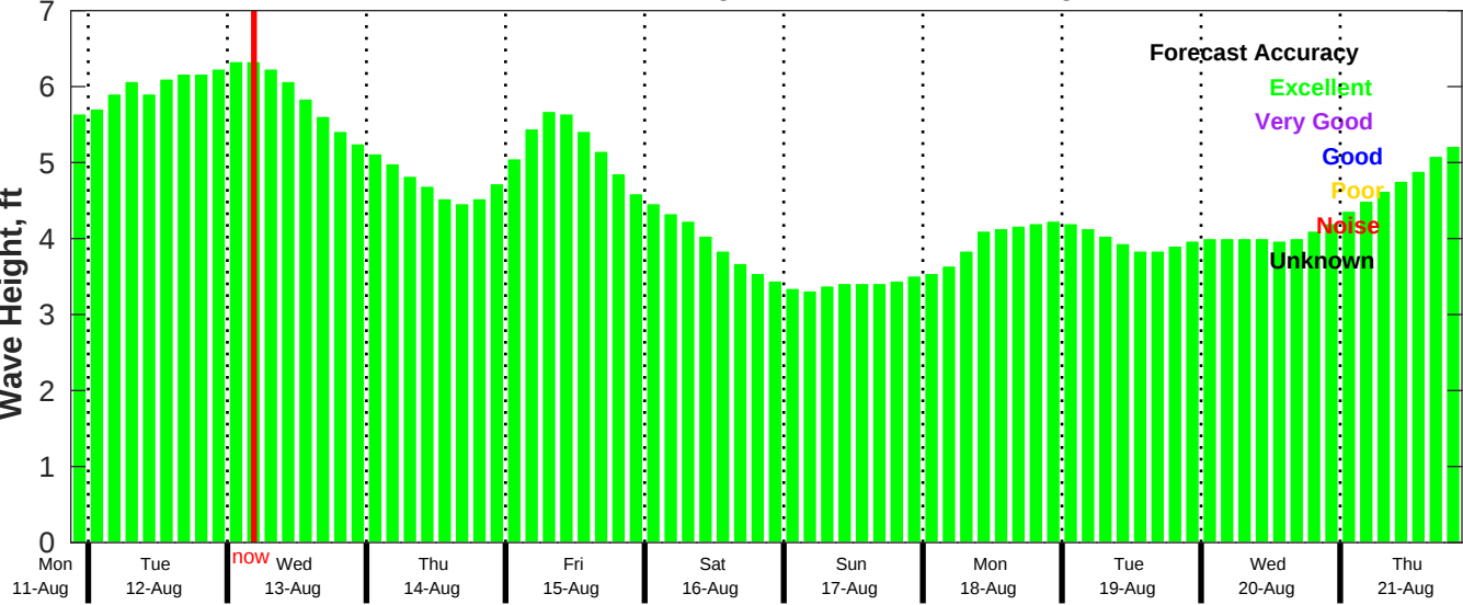
CMEMS Wave Forecast for NDBC 41040 from 11-Aug-2025 21:00:00 to 21-Aug-2025 21:00:00
