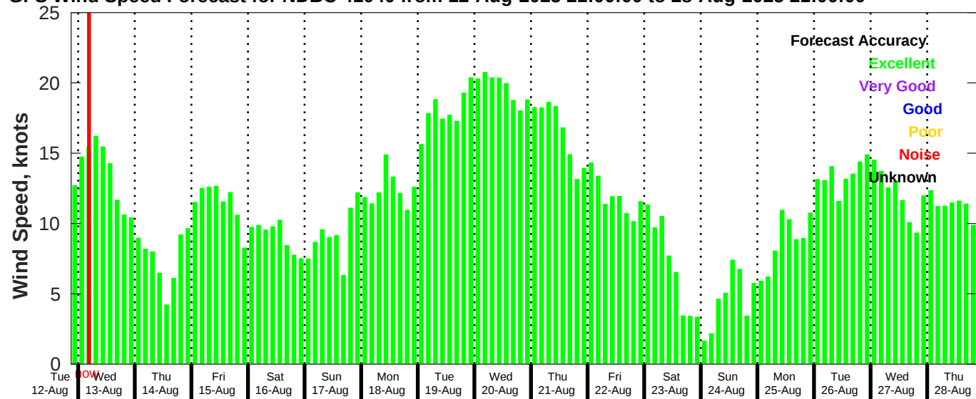
GFS Wind Speed Forecast for NDBC 41040 from 12-Aug-2025 21:00:00 to 28-Aug-2025 21:00:00
