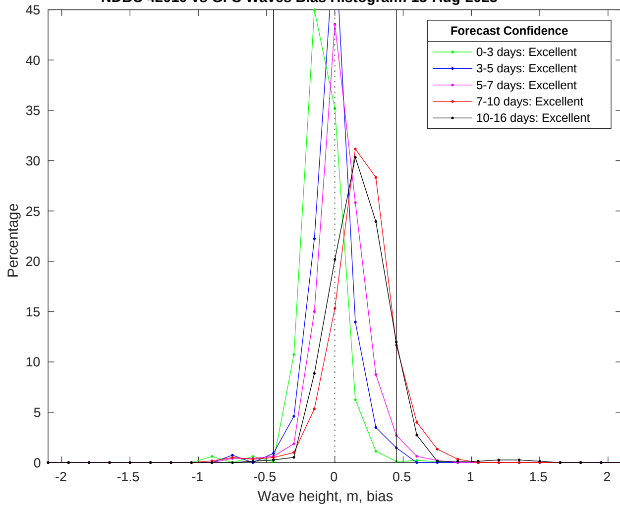
NDBC 42019 vs GFS Waves Bias Histogram: 13-Aug-2025
