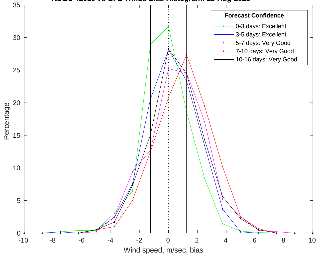
NDBC 42019 vs GFS Winds Bias Histogram: 13-Aug-2025
