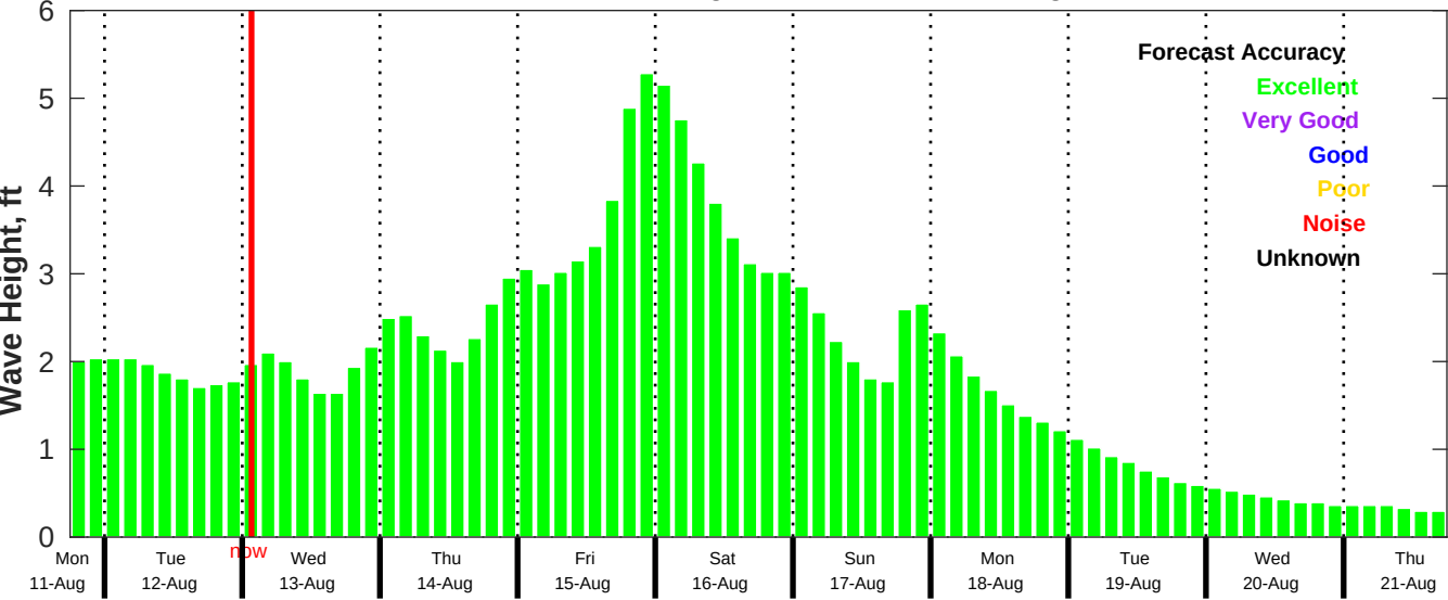
CMEMS Wave Forecast for NDBC 42020 from 11-Aug-2025 18:00:00 to 21-Aug-2025 18:00:00
