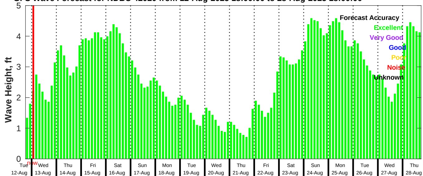
GFS Wave Forecast for NDBC 42020 from 12-Aug-2025 18:00:00 to 28-Aug-2025 18:00:00
