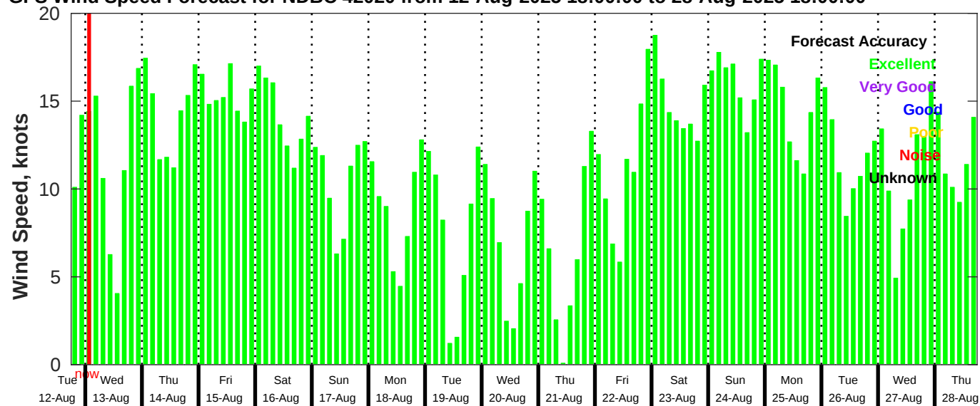
GFS Wind Speed Forecast for NDBC 42020 from 12-Aug-2025 18:00:00 to 28-Aug-2025 18:00:00
