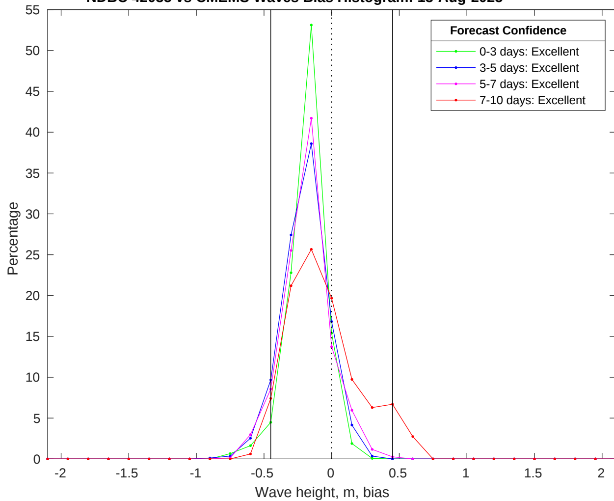
NDBC 42035 vs CMEMS Waves Bias Histogram: 13-Aug-2025
