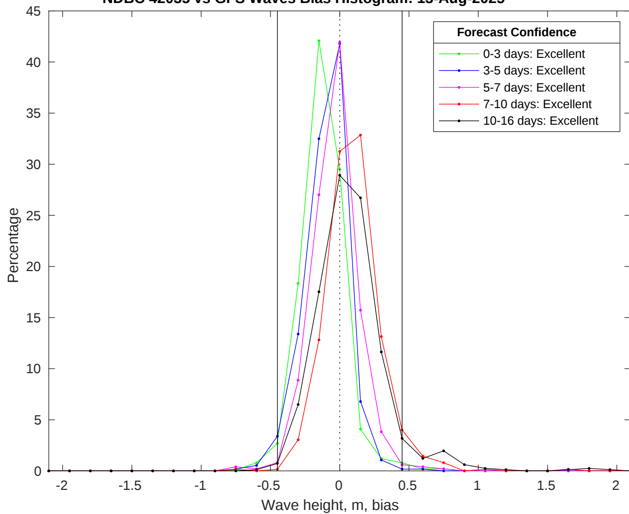
NDBC 42035 vs GFS Waves Bias Histogram: 13-Aug-2025
