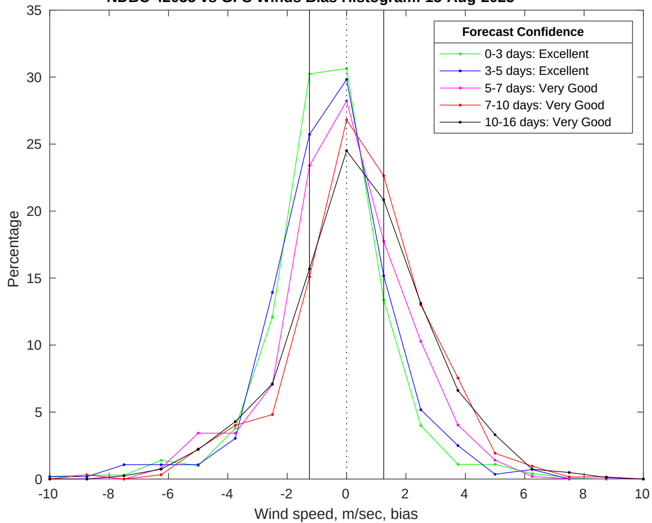
NDBC 42035 vs GFS Winds Bias Histogram: 13-Aug-2025
