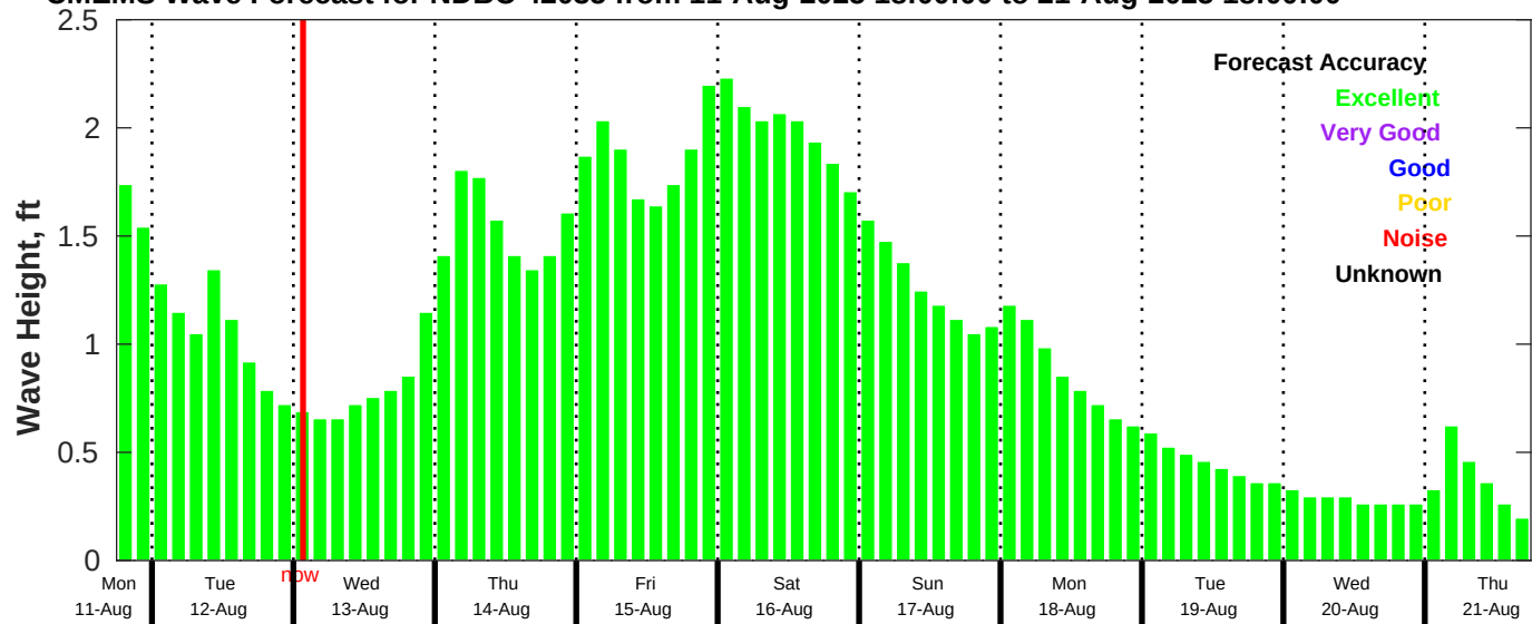
CMEMS Wave Forecast for NDBC 42035 from 11-Aug-2025 18:00:00 to 21-Aug-2025 18:00:00
