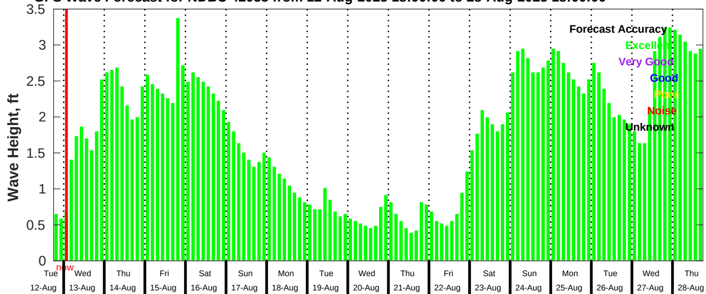
GFS Wave Forecast for NDBC 42035 from 12-Aug-2025 18:00:00 to 28-Aug-2025 18:00:00
