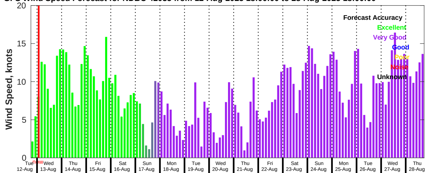
GFS Wind Speed Forecast for NDBC 42035 from 12-Aug-2025 18:00:00 to 28-Aug-2025 18:00:00
