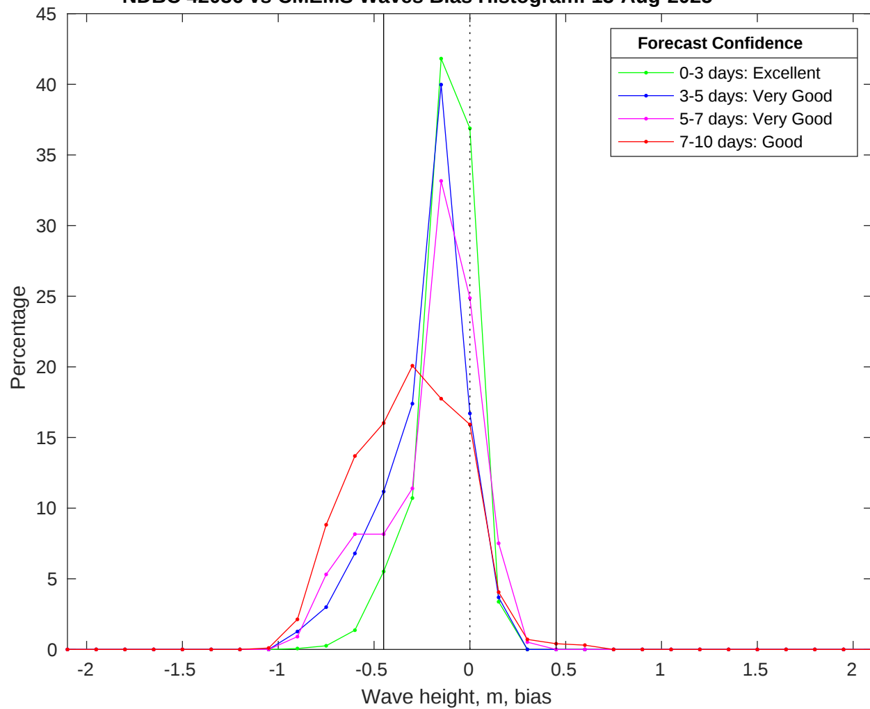
NDBC 42036 vs CMEMS Waves Bias Histogram: 13-Aug-2025
