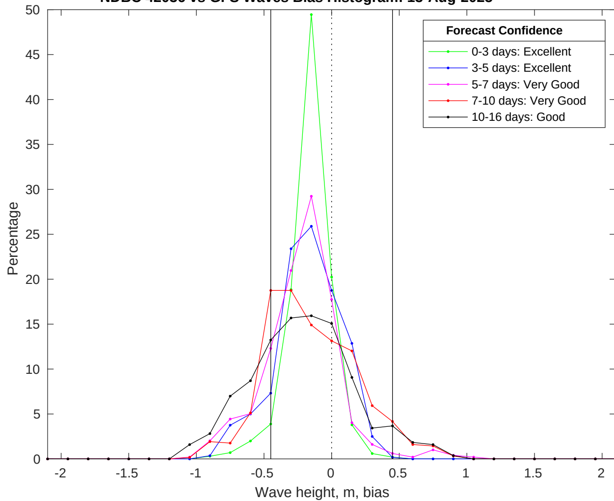
NDBC 42036 vs GFS Waves Bias Histogram: 13-Aug-2025
