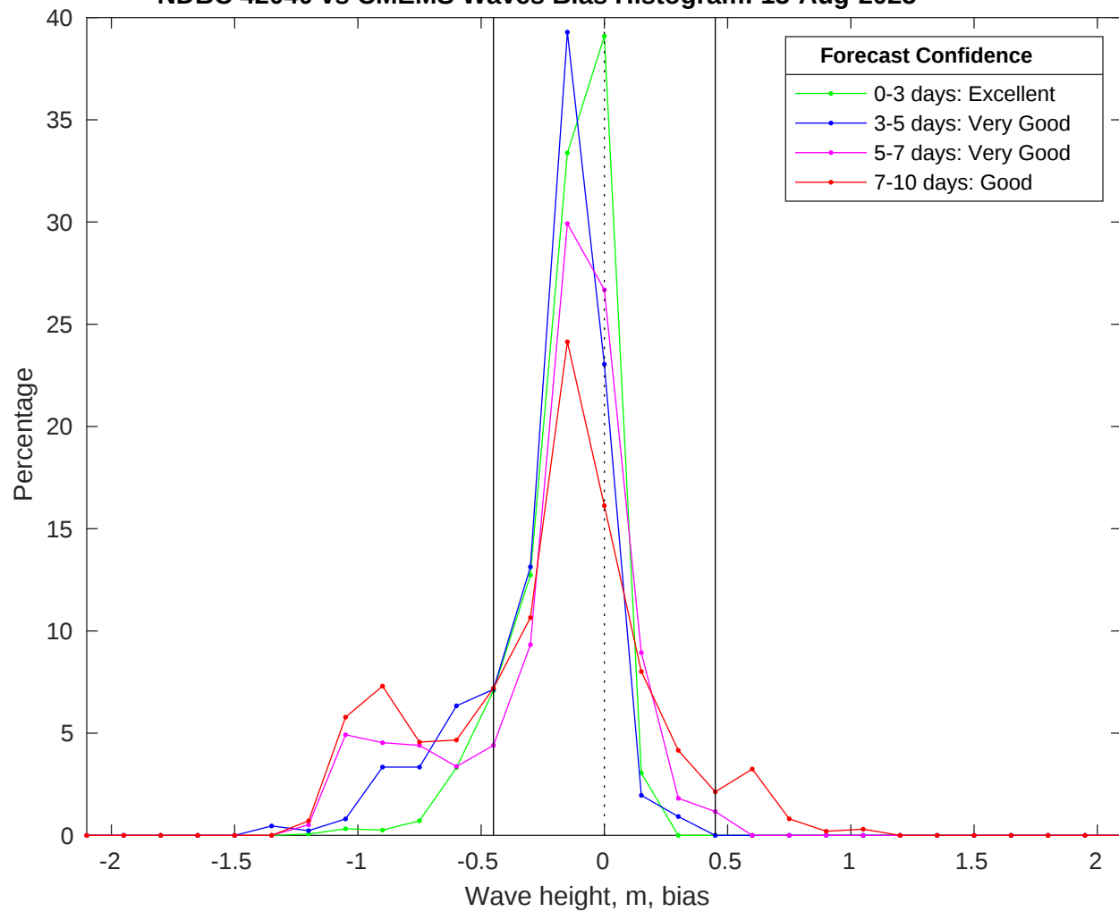
NDBC 42040 vs CMEMS Waves Bias Histogram: 13-Aug-2025
