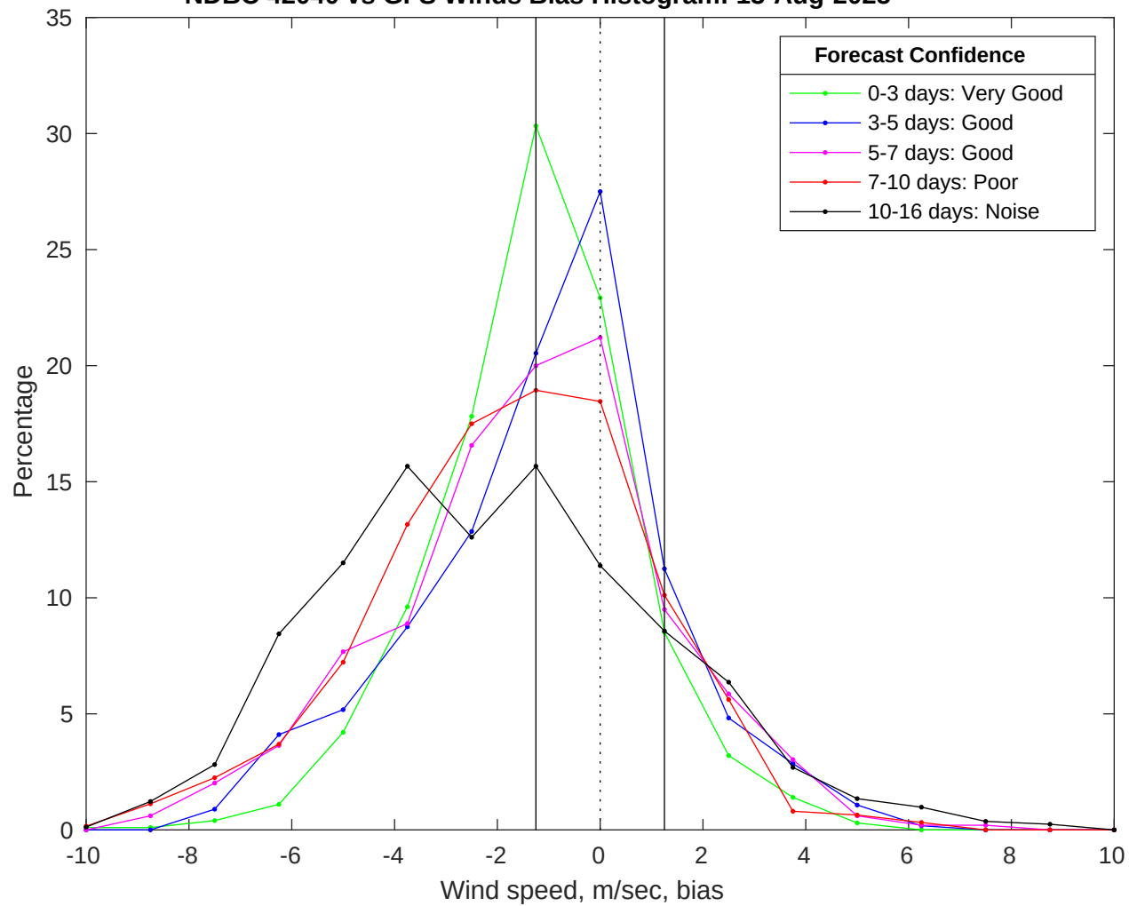
NDBC 42040 vs GFS Winds Bias Histogram: 13-Aug-2025
