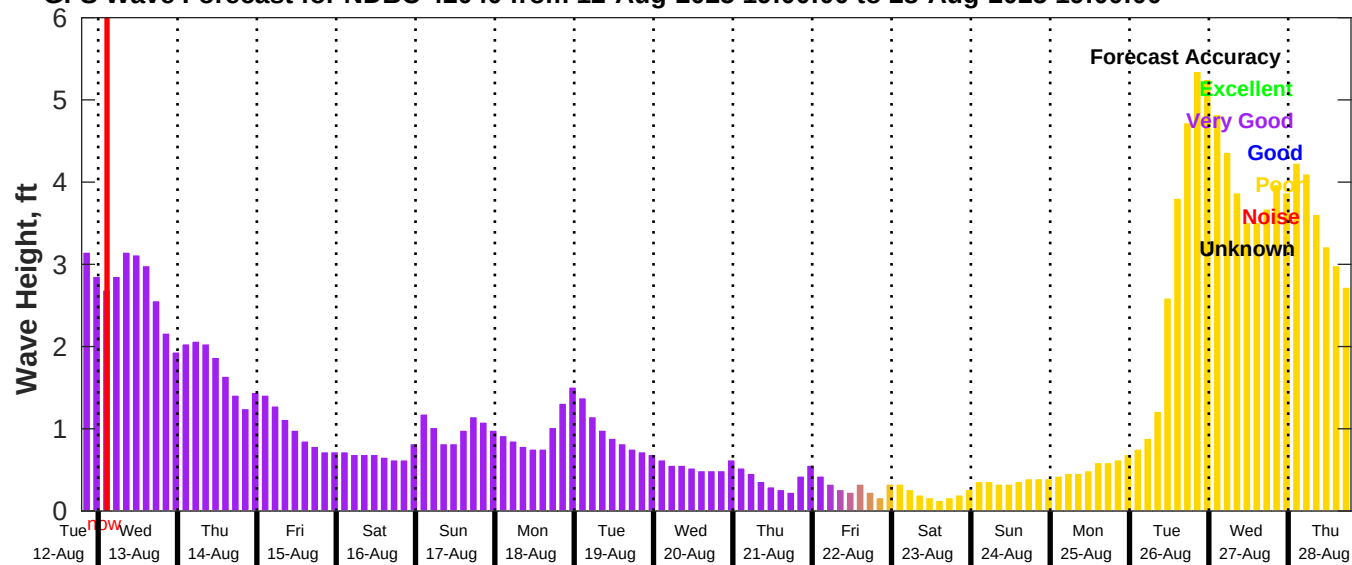
GFS Wave Forecast for NDBC 42040 from 12-Aug-2025 19:00:00 to 28-Aug-2025 19:00:00
