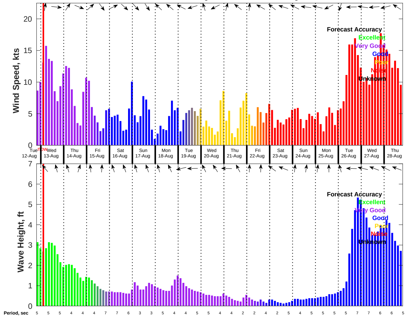
Wind & Wave Forecast for NDBC 42040 from 12-Aug-2025 19:00:00 to 28-Aug-2025 19:00:00
