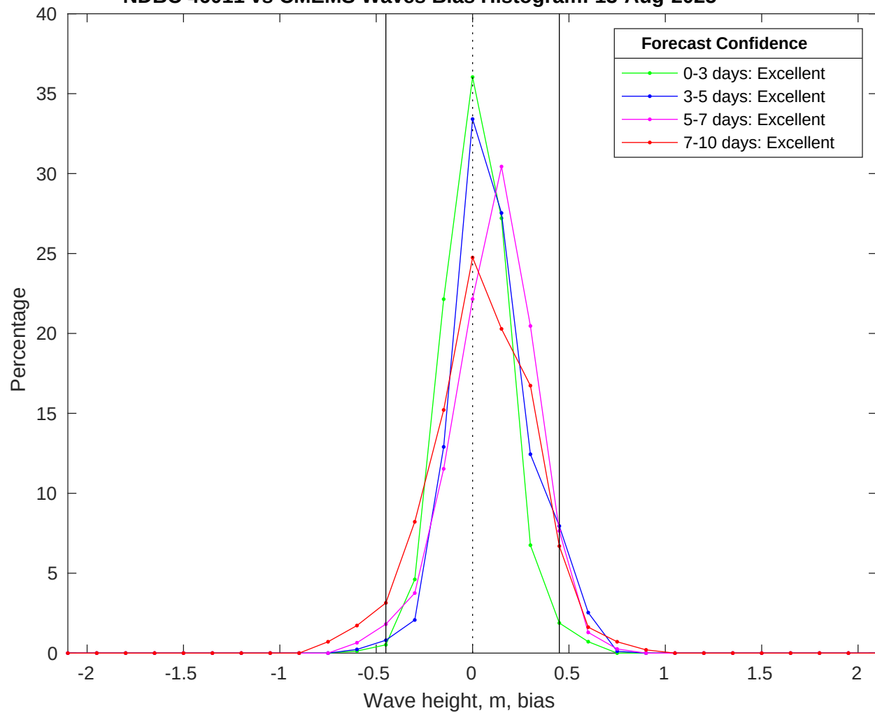
NDBC 46011 vs CMEMS Waves Bias Histogram: 13-Aug-2025
