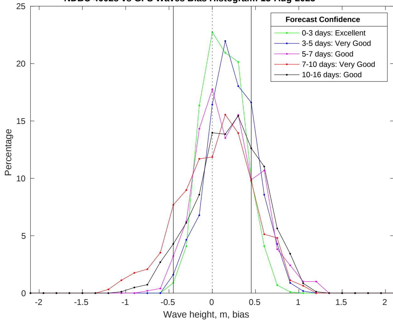
NDBC 46028 vs GFS Waves Bias Histogram: 13-Aug-2025
