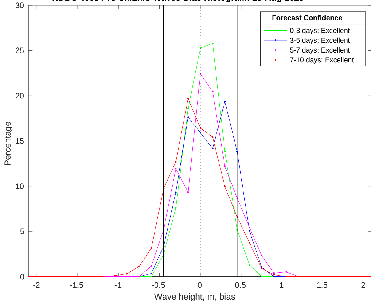
NDBC 46054 vs CMEMS Waves Bias Histogram: 13-Aug-2025
