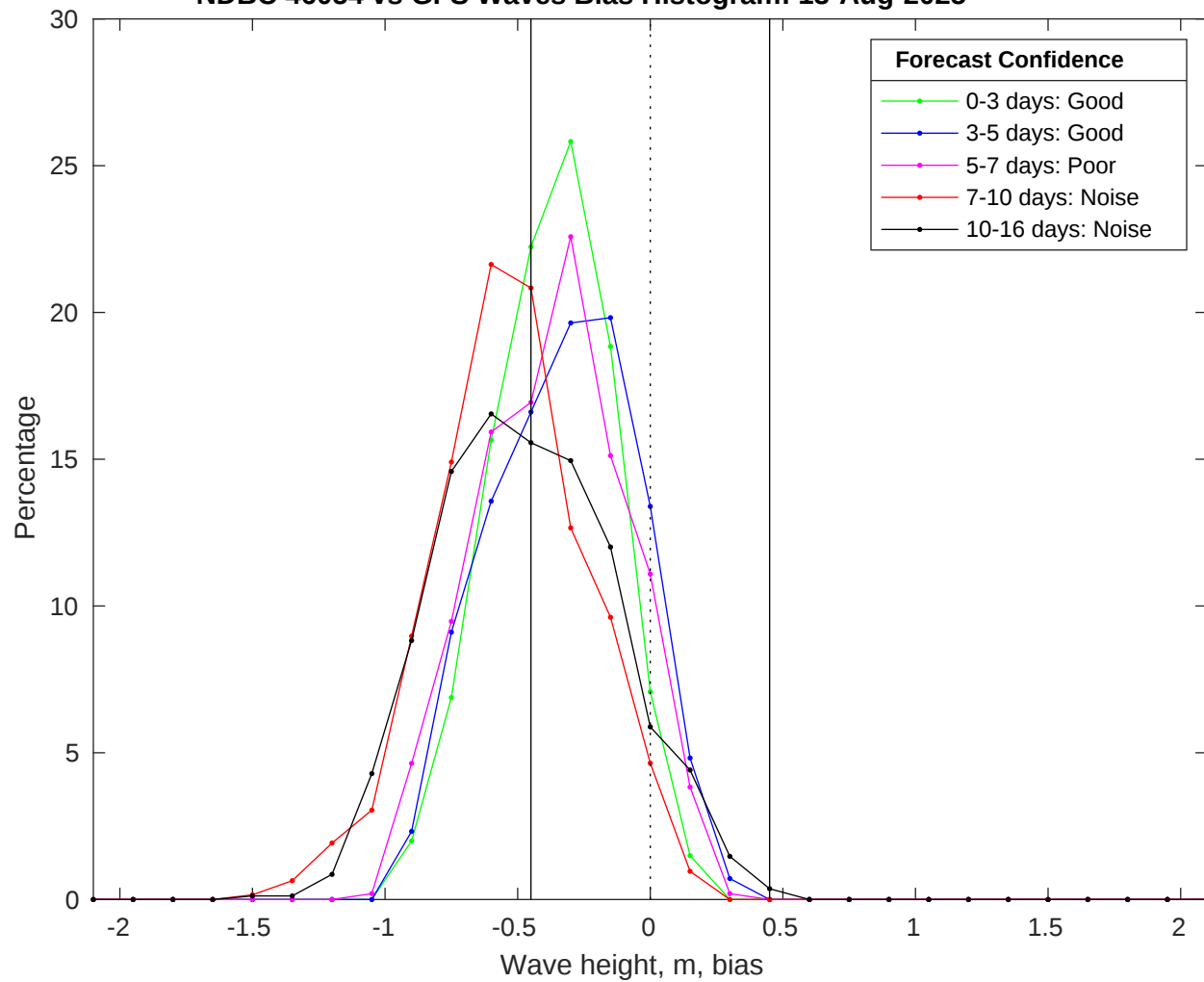
NDBC 46054 vs GFS Waves Bias Histogram: 13-Aug-2025
