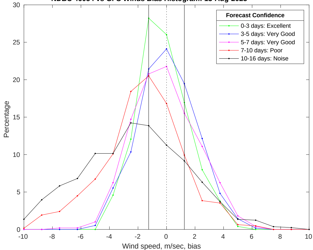
NDBC 46054 vs GFS Winds Bias Histogram: 13-Aug-2025
