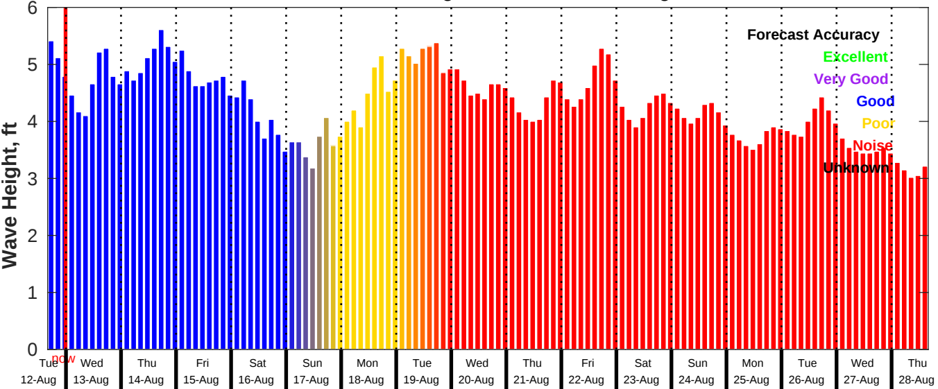
GFS Wave Forecast for NDBC 46054 from 12-Aug-2025 16:00:00 to 28-Aug-2025 16:00:00
