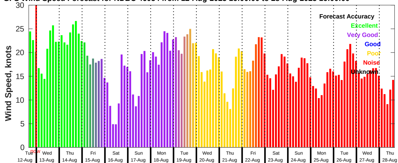
GFS Wind Speed Forecast for NDBC 46054 from 12-Aug-2025 16:00:00 to 28-Aug-2025 16:00:00
