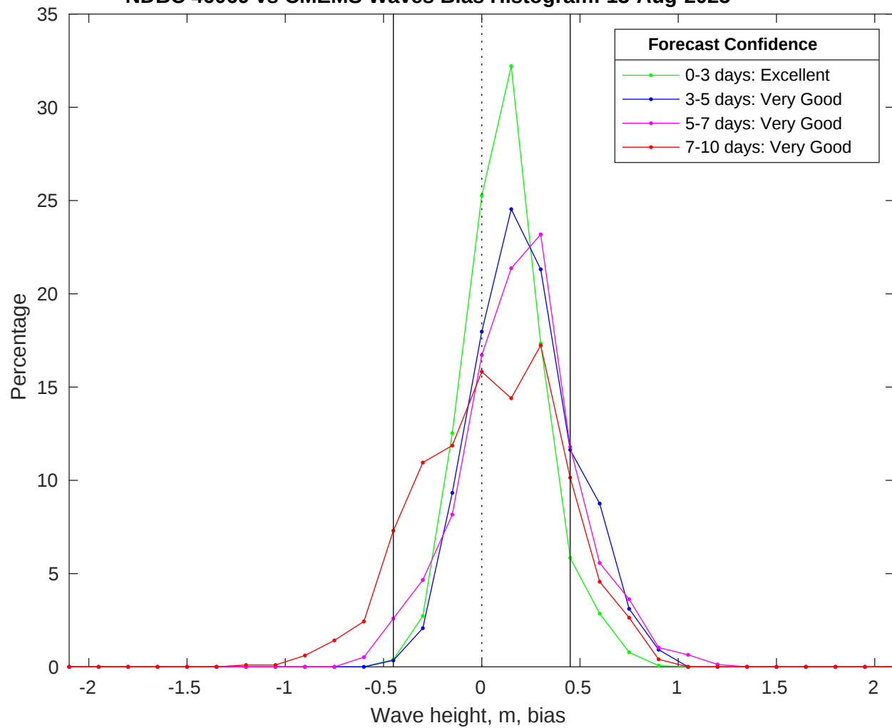
NDBC 46069 vs CMEMS Waves Bias Histogram: 13-Aug-2025
