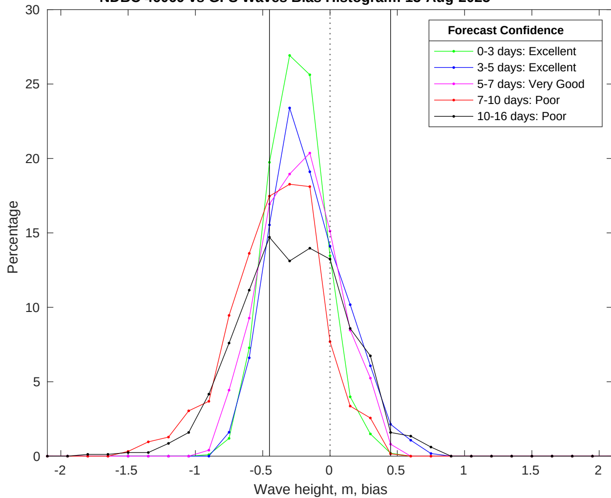
NDBC 46069 vs GFS Waves Bias Histogram: 13-Aug-2025
