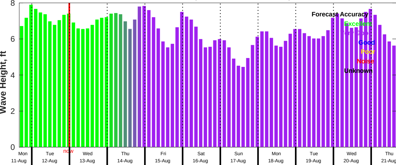
CMEMS Wave Forecast for NDBC 46069 from 11-Aug-2025 16:00:00 to 21-Aug-2025 16:00:00
